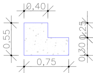
Figure 10 - Cross-section of longitudinal and transverse beams, measurements in meters.
